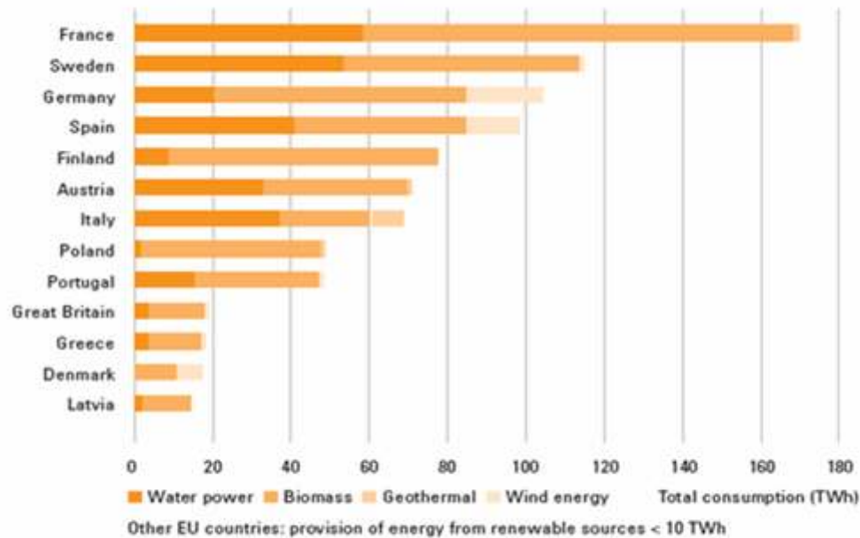
Use of renewable energy in selected EU countries in 2003
